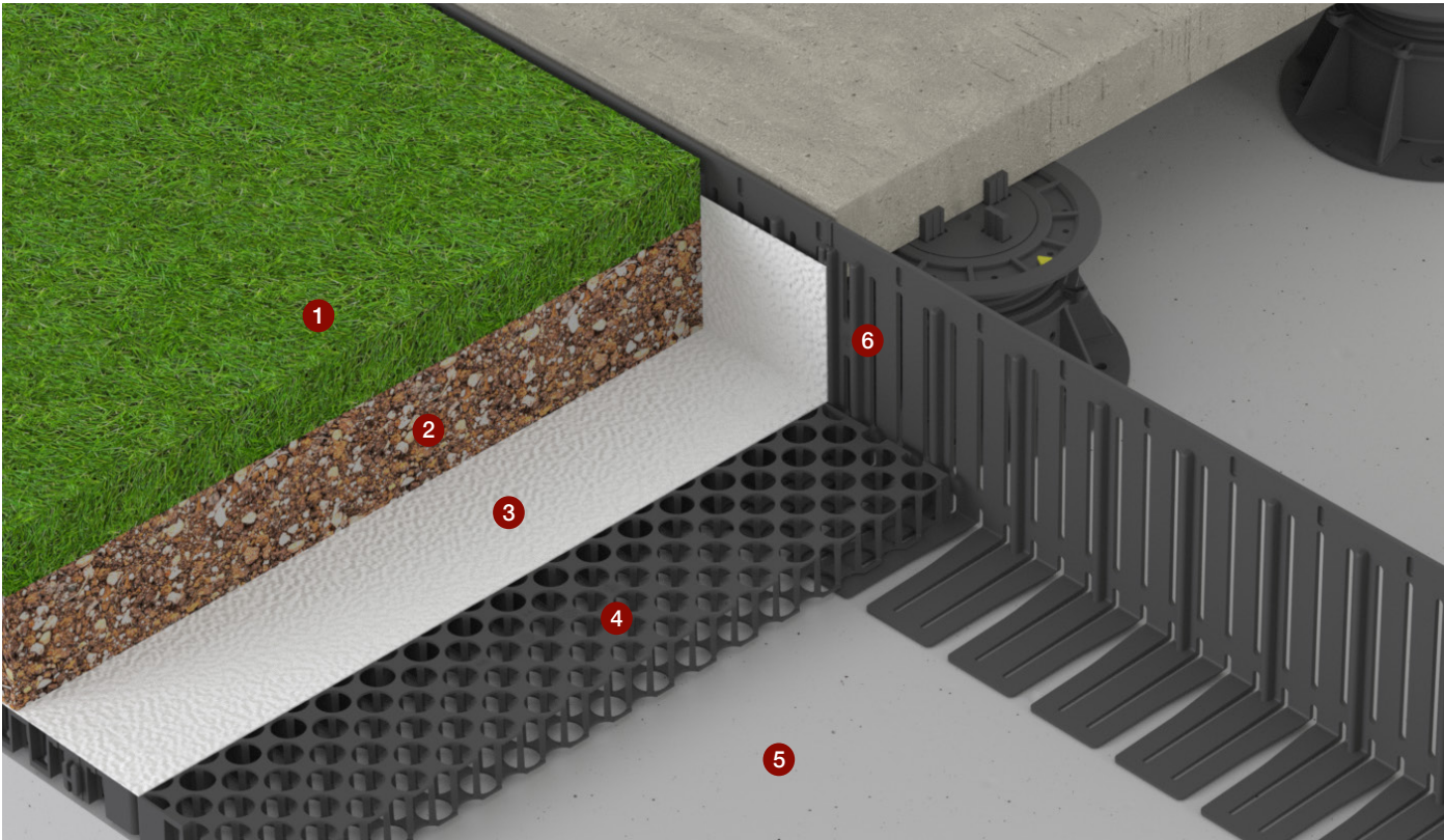
1 Turf/Plants 2 Planting Media 3 Geotextile Filter Fabric 4 VersiCell® 5 R.C Roof Slab 6 VersiEdge™ P
